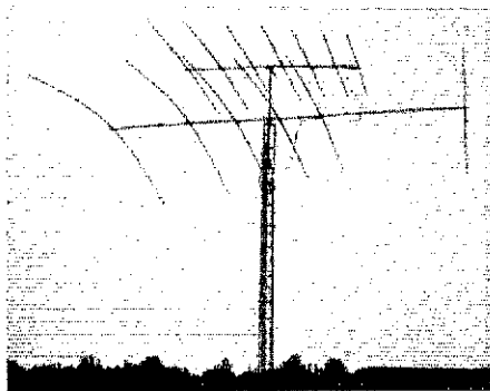
The completed Log-Yag array ready for use. The array mounted above the Log-Yag is a 7-element LPDA for 21 to 30 MHz.
